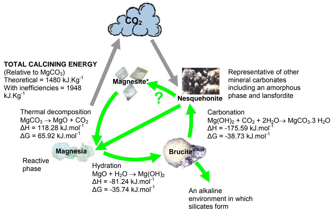
Figure 1 - The Magnesium Thermodynamic Cycle
