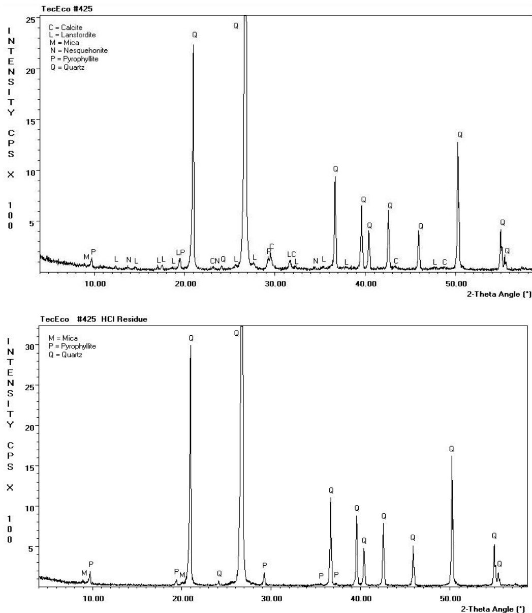
Figure 2 - XRD Showing Carbonates Before and Minerals Remaining after their Removal with HCl in a Simple Mix (70 Kg PC, 70 Kg MgO, colouring oxide .5Kg, sand unwashed 1105 Kg)
